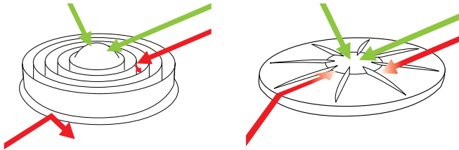
1) Choke Ring weakens multipath signals
